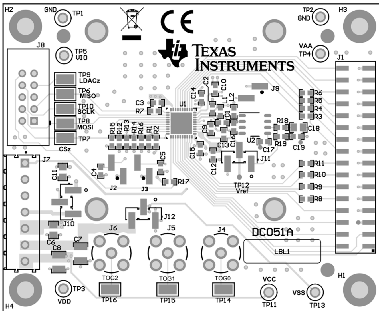
Figure 13. DAC81408EVM PCB Components Layout
