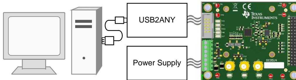
Figure 1. DAC81408EVM Hardware Setup
