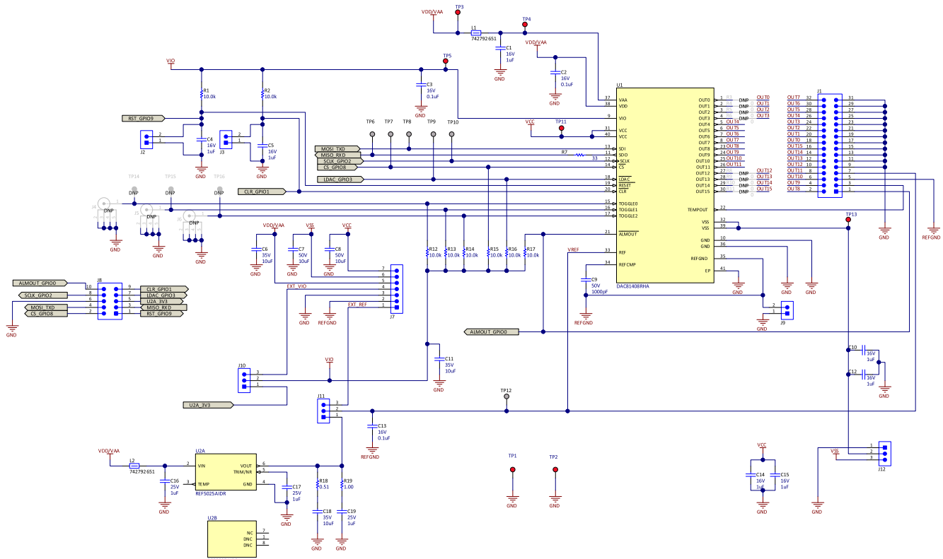
Figure 12. DAC81408EVM Board Schematic
