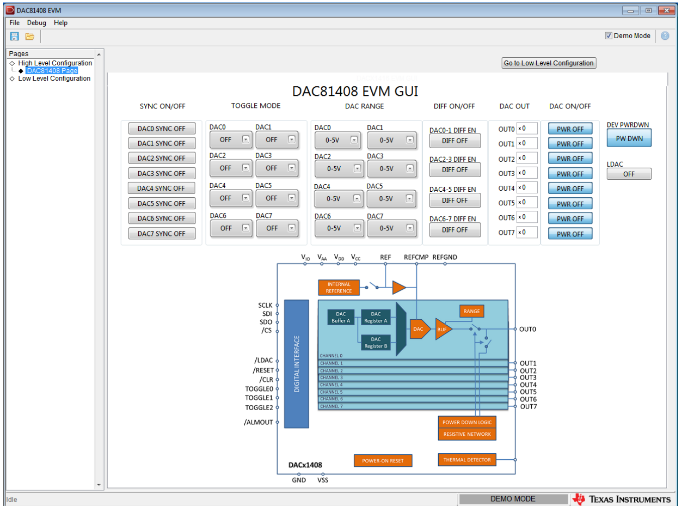
Figure 11. High Level Configuration Page
