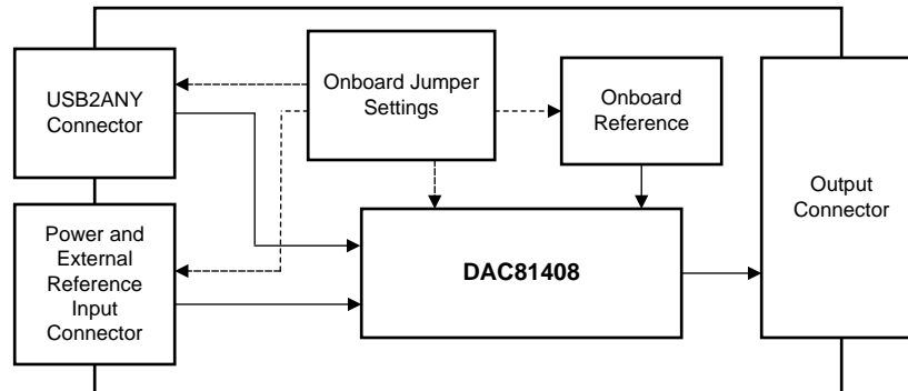
Figure 4. DAC81408EVM Hardware Block Diagram
