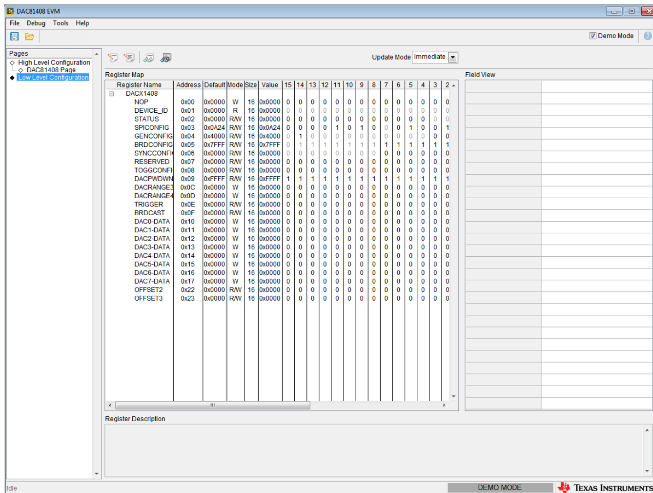
Figure 9. Low Level Configuration Page
